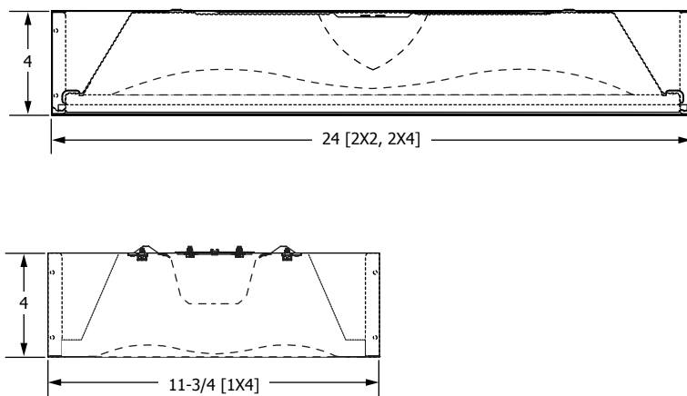
END VIEWS
