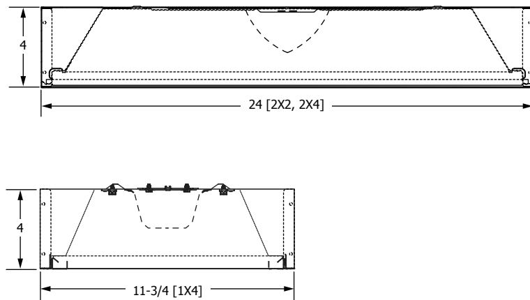
END VIEWS
