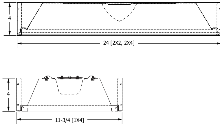
END VIEWS
