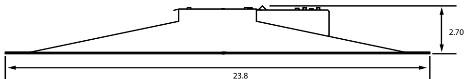
END VIEW
